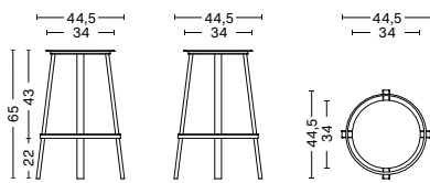
REVOLVER BAR STOOL LOW HEIGHT 65 CM | 25.50" DIAMETER BASE 44,5 CM | 17.50" DIAMETER SEAT 34 CM | 13.50"
