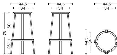
REVOLVER BAR STOOL HIGH HEIGHT 76 CM | 30" DIAMETER BASE 44,5 CM | 17.50" DIAMETER SEAT 34 CM | 13.50"
